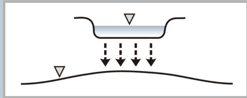
Infiltration basin
